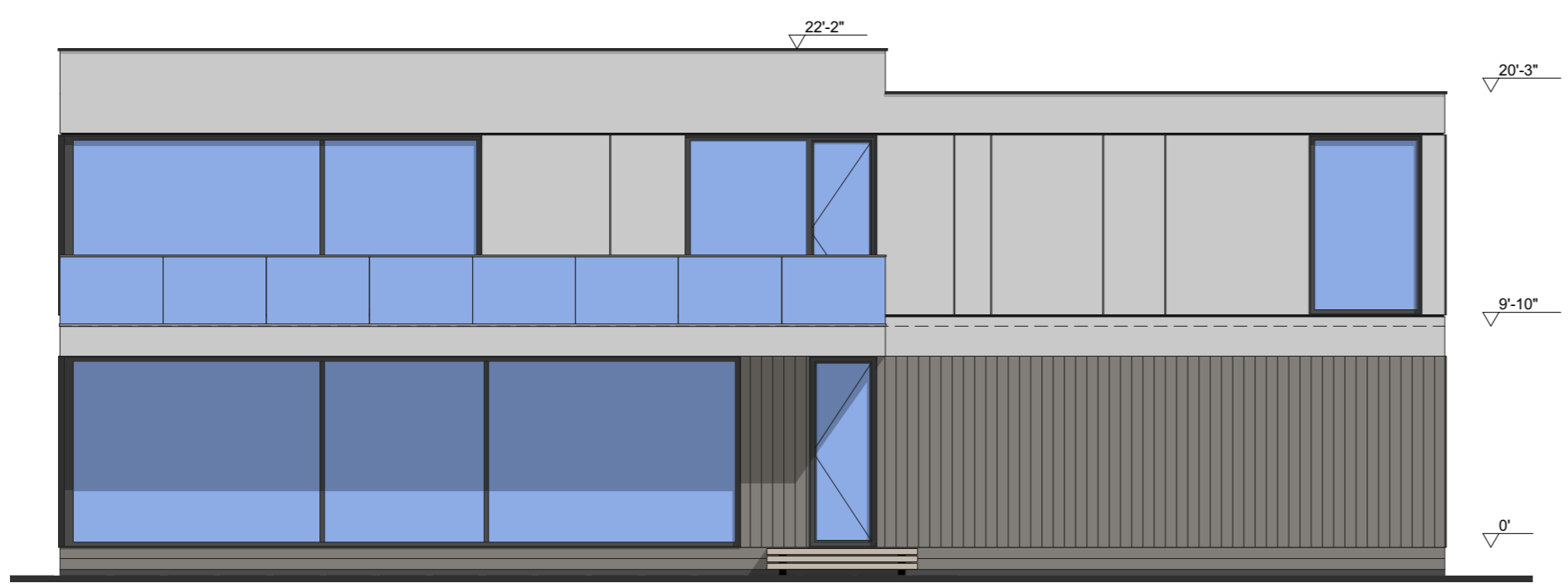
SOUTH ELEVATION
